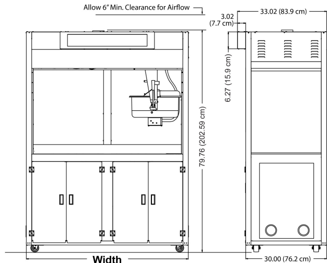
60" Cabinet shown for dimension reference only.
